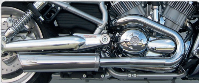
Fits 2002 thru 2017 V-Rod 749949 Fits V-Rod Muscle 749950 2-into-1 slip-on muffler for 2002 thru 2017 V-Rod except Muscle 749951 Slip-on mufflers for 2002 thru 2017 V-Rod except Muscle 749952 Optional adjusting motor with remote control
